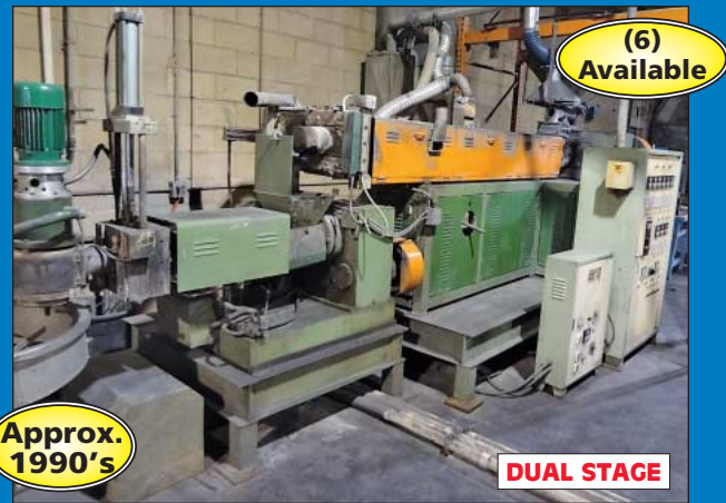
(6) 6" Continental Polymer Pelletizing Lines w/ Single and Dual State Extruders, Spin Dryers and Pelletizers
