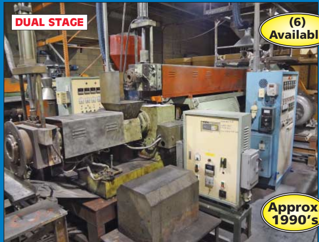
(6) 6" Continental Polymer Pelletizing Lines w/ Single and Dual State Extruders, Spin Dryers and Pelletizers
