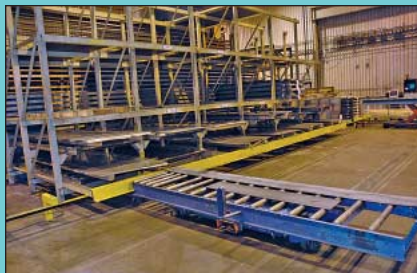
9'D X 30'W X 13' High Fabricated Steel Roller Shelf Rack w/ (2) Electric/Hydraulic Scissor Lift Tables
