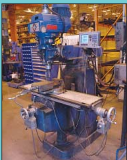
3 HP Hurco Model SMI Vertical Milling Machine
