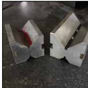
Precision Parallel, Angle & Saddle Blocks
