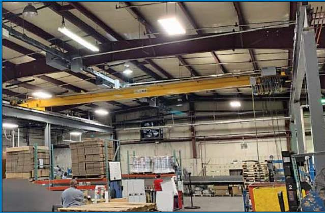
5 Ton x 40' Span X 70' Long US Crane and Hoist Free-Standing Top Running Bridge Crane System
