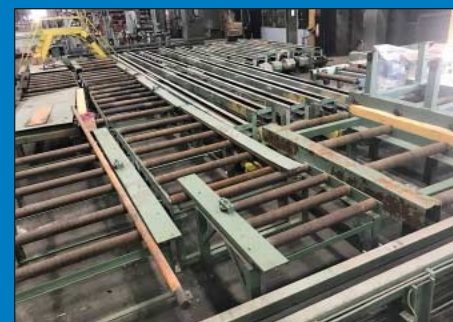
Peddinghaus Structural Conveyor
