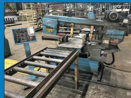
9' x 16' DoAll Model C-916DS Mitre Base Horizontal Band Saw
