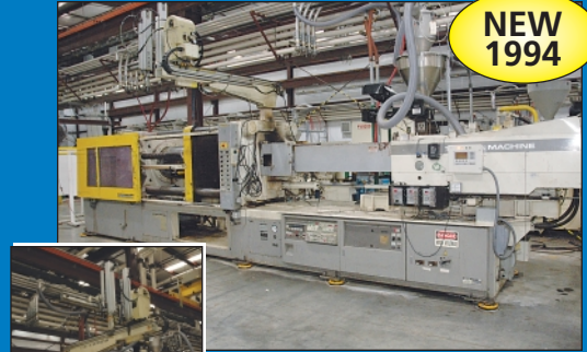
610 Ton X 124 Oz. Toshiba Model ISF610S-59B Hydraulic Clamp Plastic Injection Molding Machine
