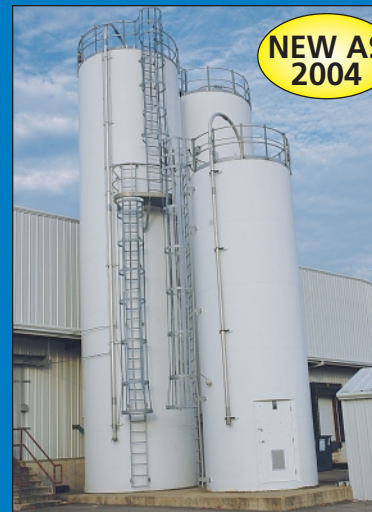
Partial View (3 of 5) Material Storage Silos To 12' X 48'
