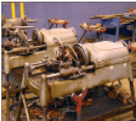
RIDGID 535 PIPE THREADERS
