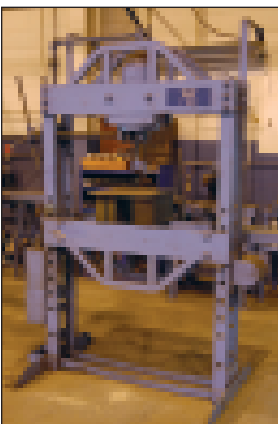
KR WILSON 37F 75-TON STRAIGHTENING PRESS
