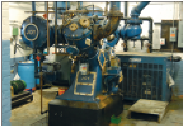
JOY WN112 TWIN CYLINDER AIR COMPRESSOR
