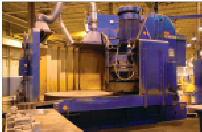
BLANCHARD 36HD66 66" ROTARY SURFACE GRINDER
