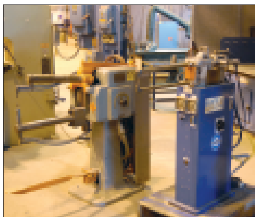
THOMPSON 25-KVA & MILLAR 10-KVA RESISTANCE WELDERS
