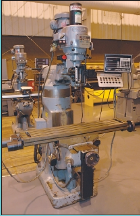
2 HP Bridgeport Two-Axis Proto-Trak CNC Vertical Milling Machine
