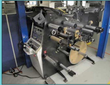
10" Rotoflex Model VSI/VLI250 Inspection / Slitter / Rewinding Machine
