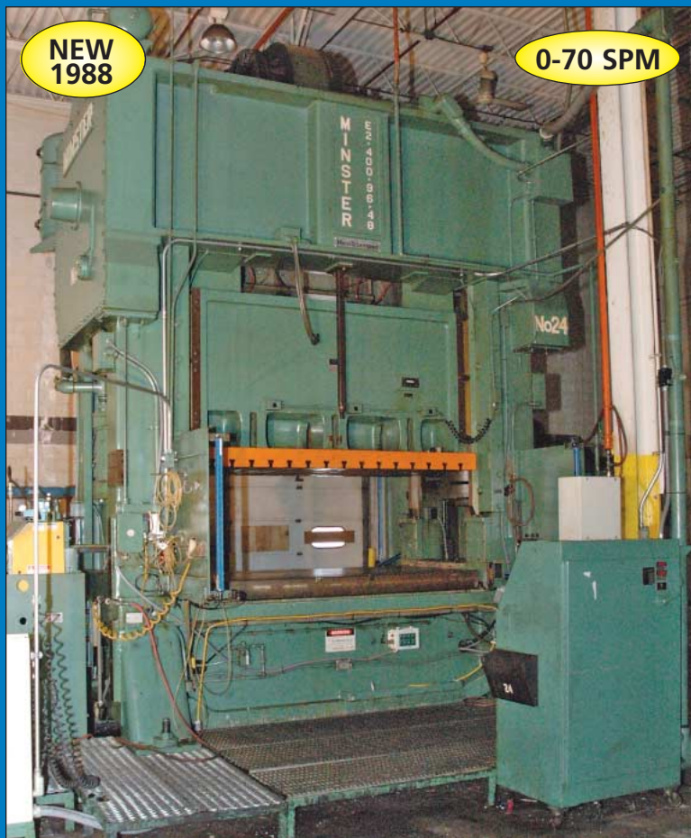
400 Ton Minster Model E2-400-96-48 Straight Side Double Crank Press
