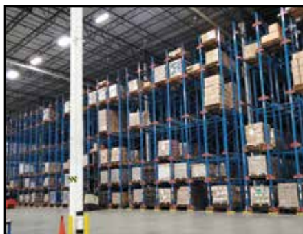
RAYMOND Push-Back Rack Shuttle Systems w/(6,000) Pallet Spaces, Shuttles & Rechargeable Battery Systems
