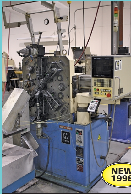
Itaya Model MCS-15G CNC Spring Winder
