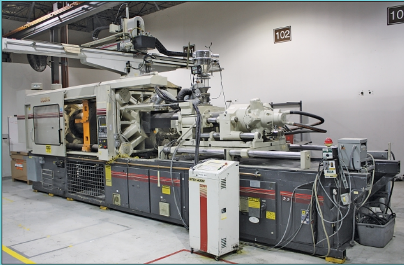
500 Ton X 68 Oz. Cincinnati Milacron Model VH500-54CE Hydraulic Clamp Plastic Injection Molding Machine
