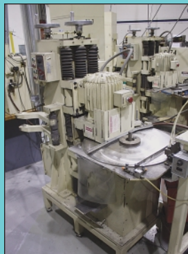
(3) Moyer Mfg. Model 12" BC Opposed Disc Spring Grinders
