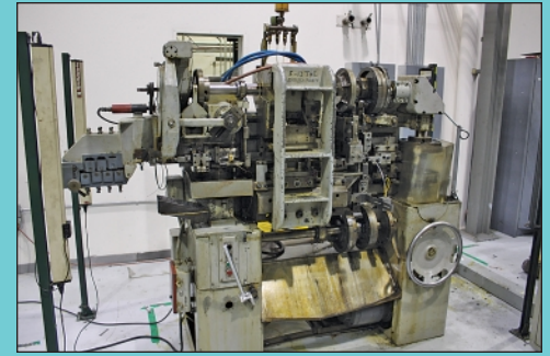
Torrington Model V-82 Verti-Slide Wire Forming Machine
